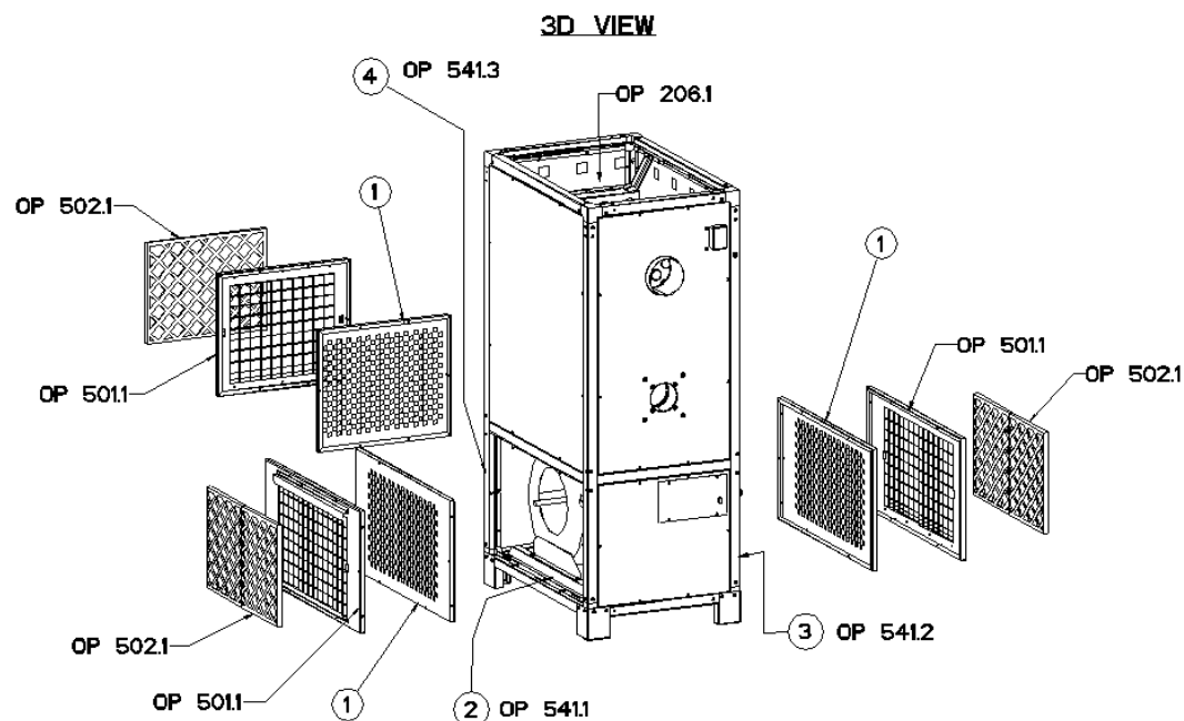
Figure 13a : Overview of the VCHE options
